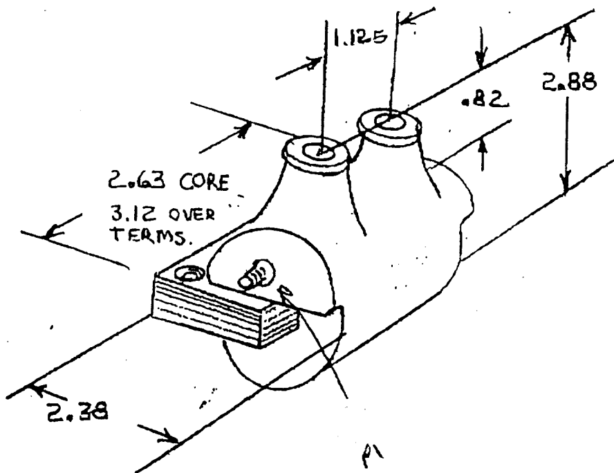
MOUNTING DETAIL
